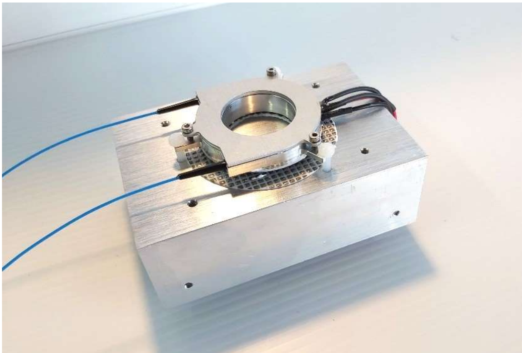
Fig. 1. OETFG-300 Thermo-Tunable FBG Filter (OEM)
